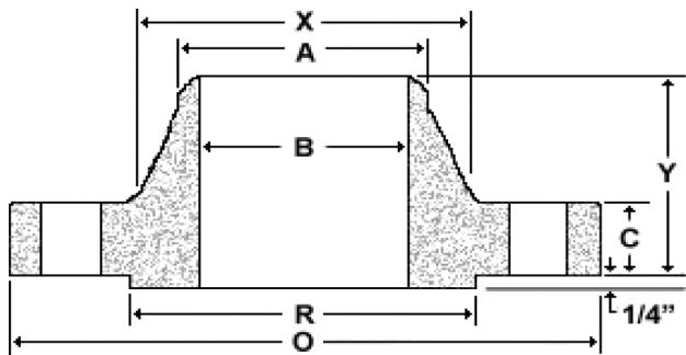
Weld Neck
